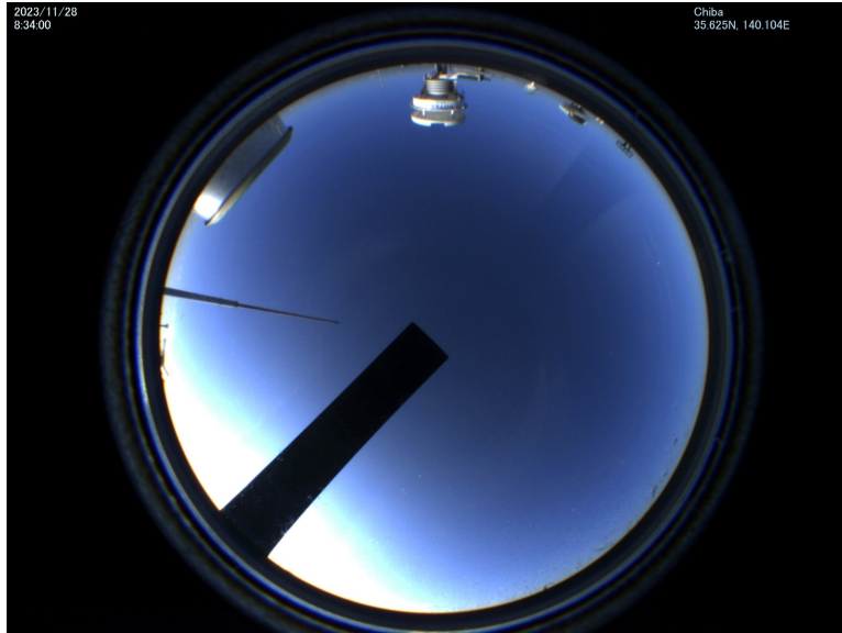
Fig1. Photo of the sky over Chiba University taken by the Skyview Camera.(8:34 AM, Nov. 28 th , 2023)
