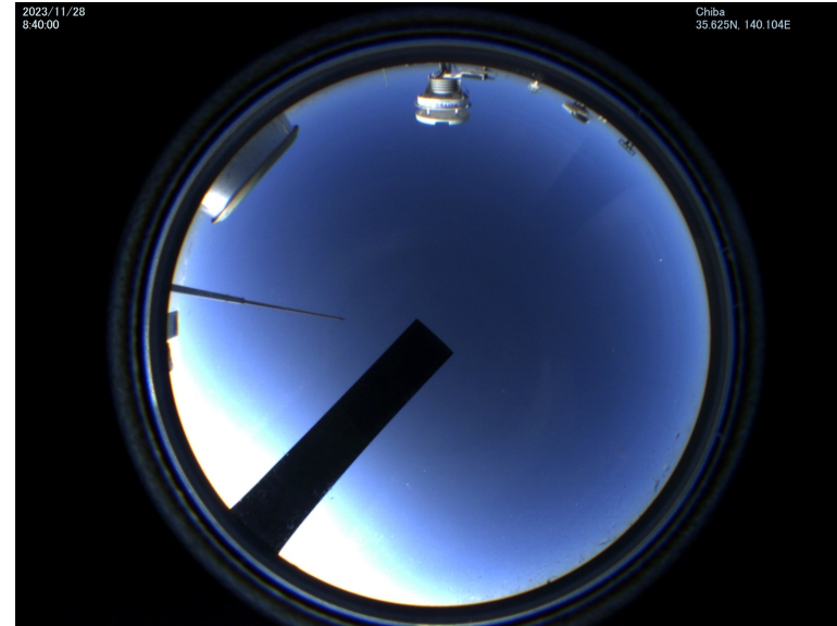
Fig2. Photo of the sky over Chiba University taken by the Skyview Camera.(8:40 AM, Nov. 28 th , 2023)
